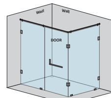
2 fixed glasses & 1 door (hinges on glass corner)
