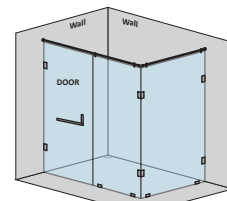
2 fixed glasses & 1 door (hinges on wall)
