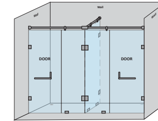
3 fixed glasses & 2 doors – shower partition (T-brackets)
