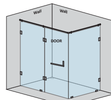
2 fixed glasses & 1 door (hinges on fix glass)
