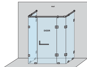
4 fixed glasses & 1 door – shower partition
