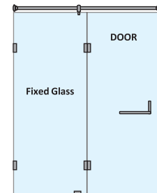
1 fixed glass & 1 door (hinges on glass)
