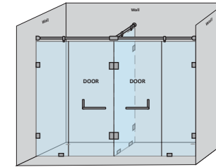
3 fixed glasses & 2 doors – shower partition (T-hinges)
