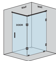
1 fixed glass & 1 door (hinges on glass corner)
